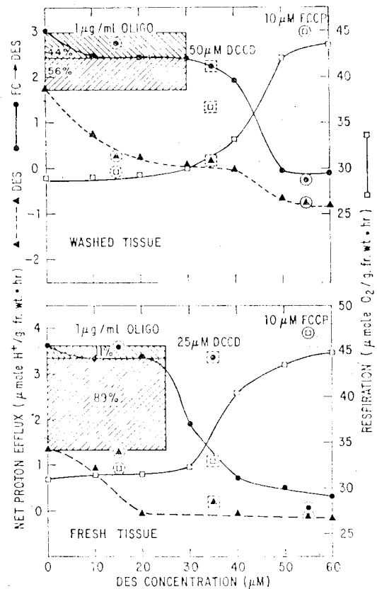
Fig. 1. Effects of DES, DCCD, oligomycin (OLIGO), and FCCP on corn root respiration (■), basal (▲) and FC-stimulated (●) net H^+ efflux. FC concentration was 20 \mu M . In fresh tissue (lower panel) 11% of FC-stimulated net H^+ efflux was DES sensitive, and 89% was DES insensitive. In washed tissue (upper panel) it was 44% and 56%, respectively. Points outlined with closed circles, dashed square and dashed circles represent the effect of FCCP, DCCD and oligomycin, respectively, in the absence of DES.
